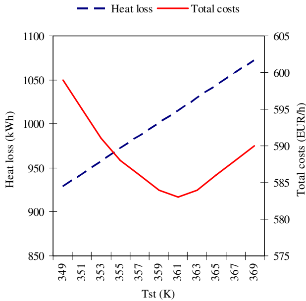
Figure 2: The connection between supply temperature, heat losses and the total costs of heat production and distribution
