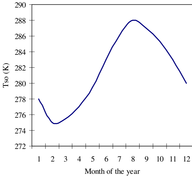
Figure 1: T_{so} at a depth of 1m, depending on the month
