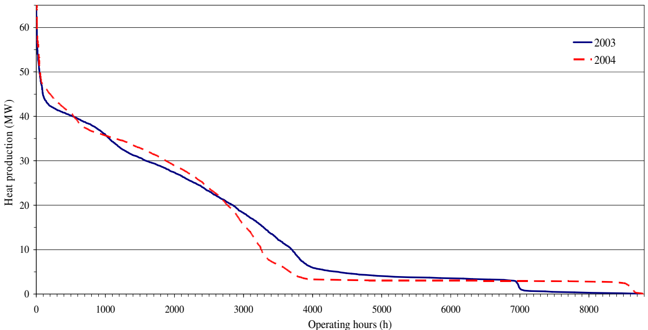
Figure 5: Hourly profile of heat production in the TOM network
