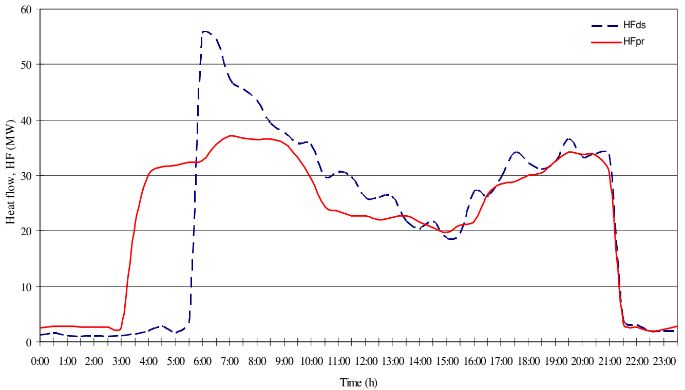
Figure 4: An example of cost-effective management of heat production and distribution at TOM
